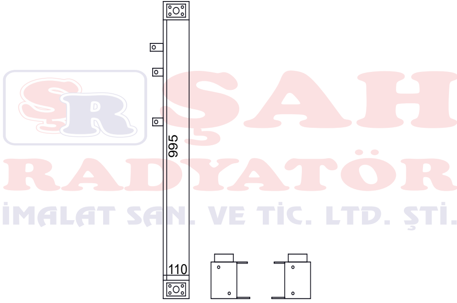
JCB 426
